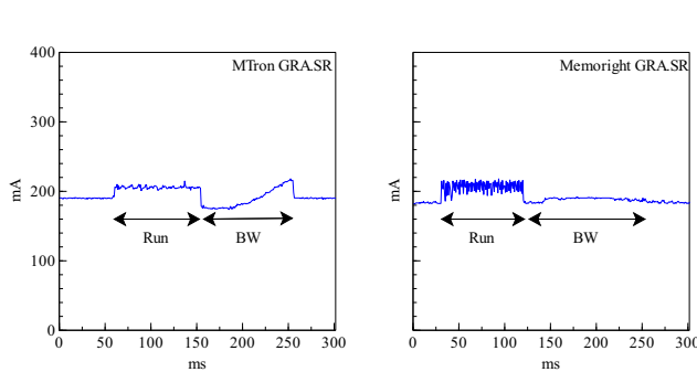
Figure 5: Systematic background work (BW) for MTron (left) and Memoright (right)
