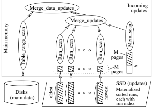
(a) MaSM algorithm using 2M memory
